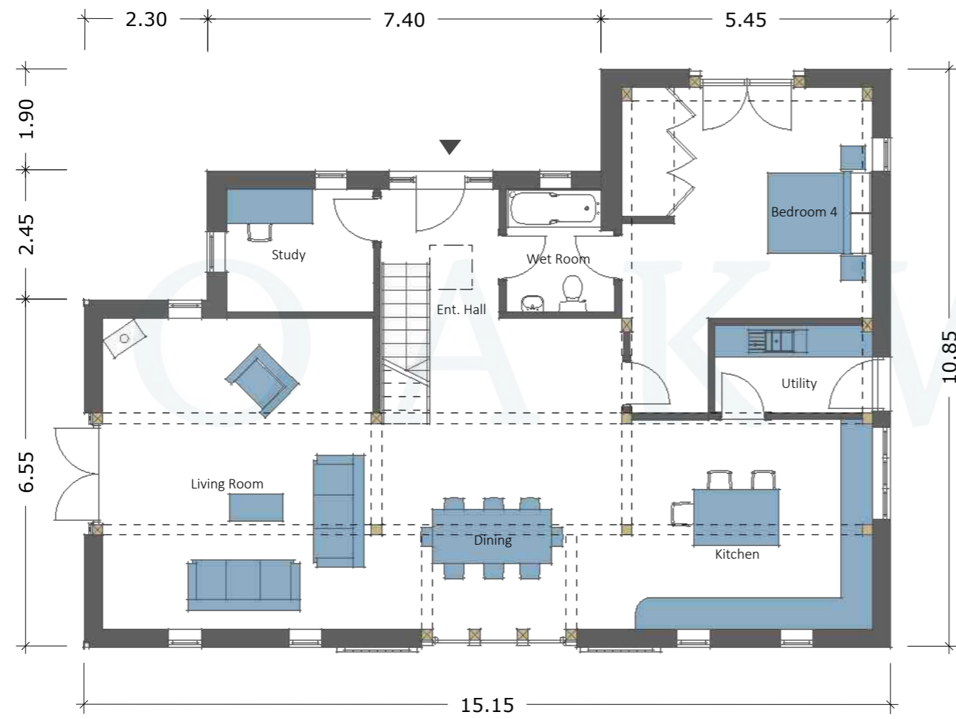
GROUND FLOOR GEA- 140.40 m 2
