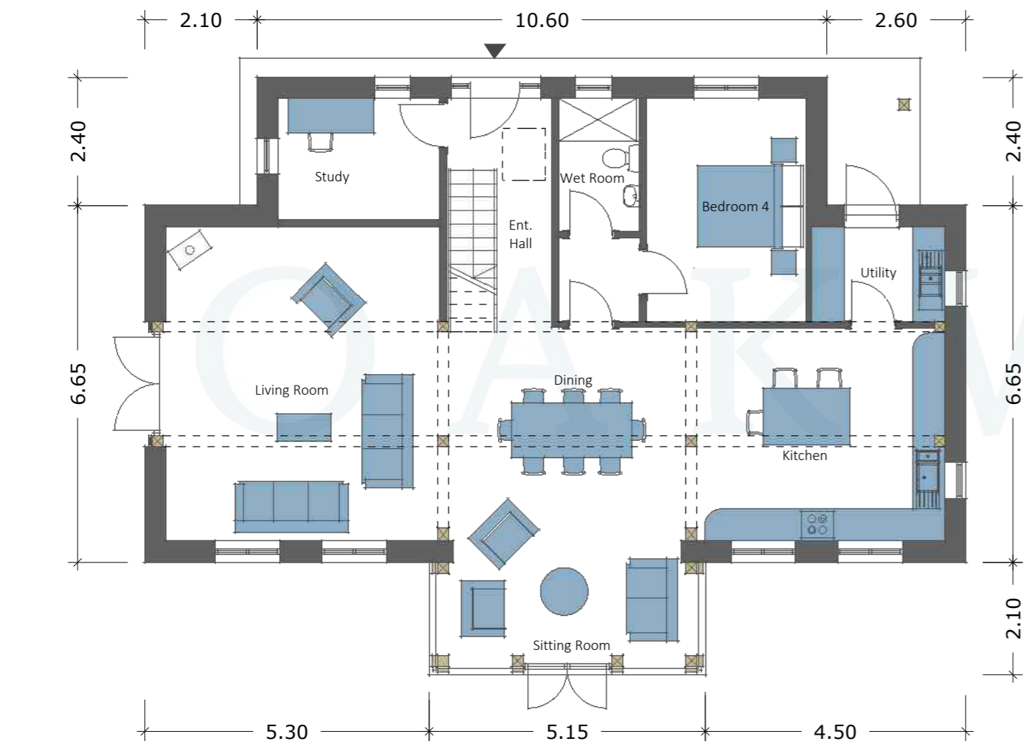
GROUND FLOOR GEA- 148.80 m 2
