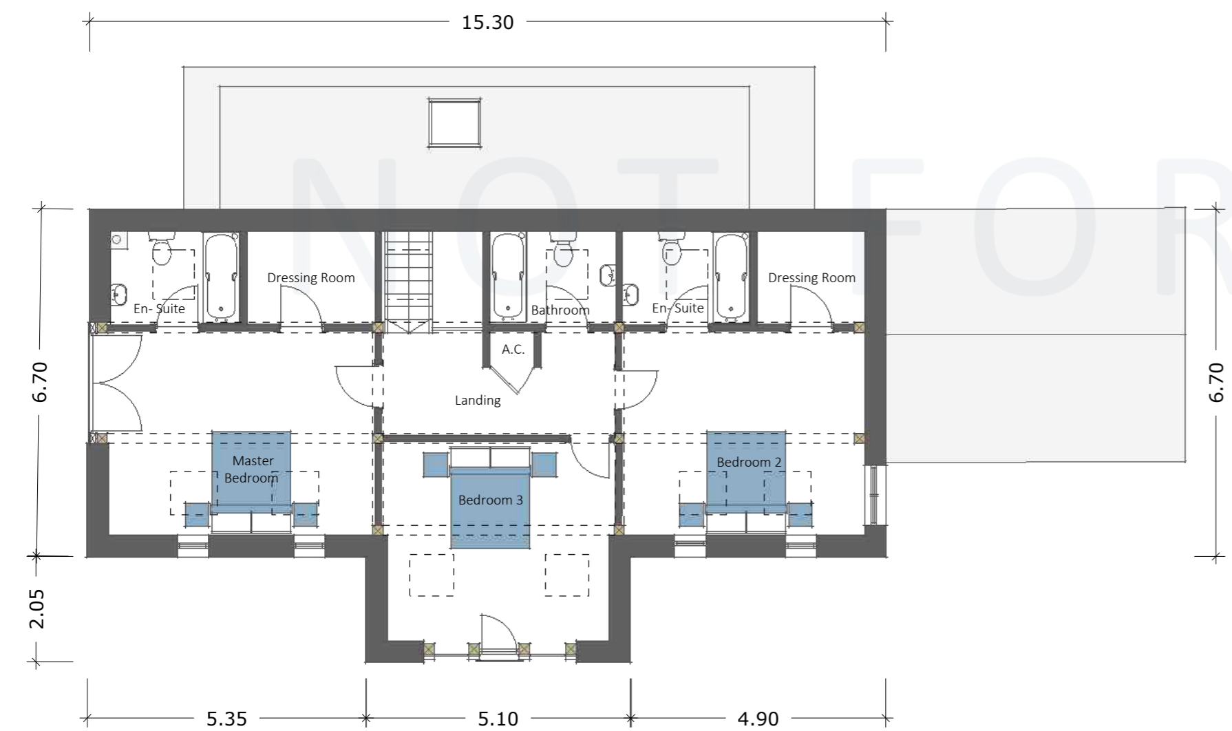
FIRST FLOOR GEA- 112.20 m 2
