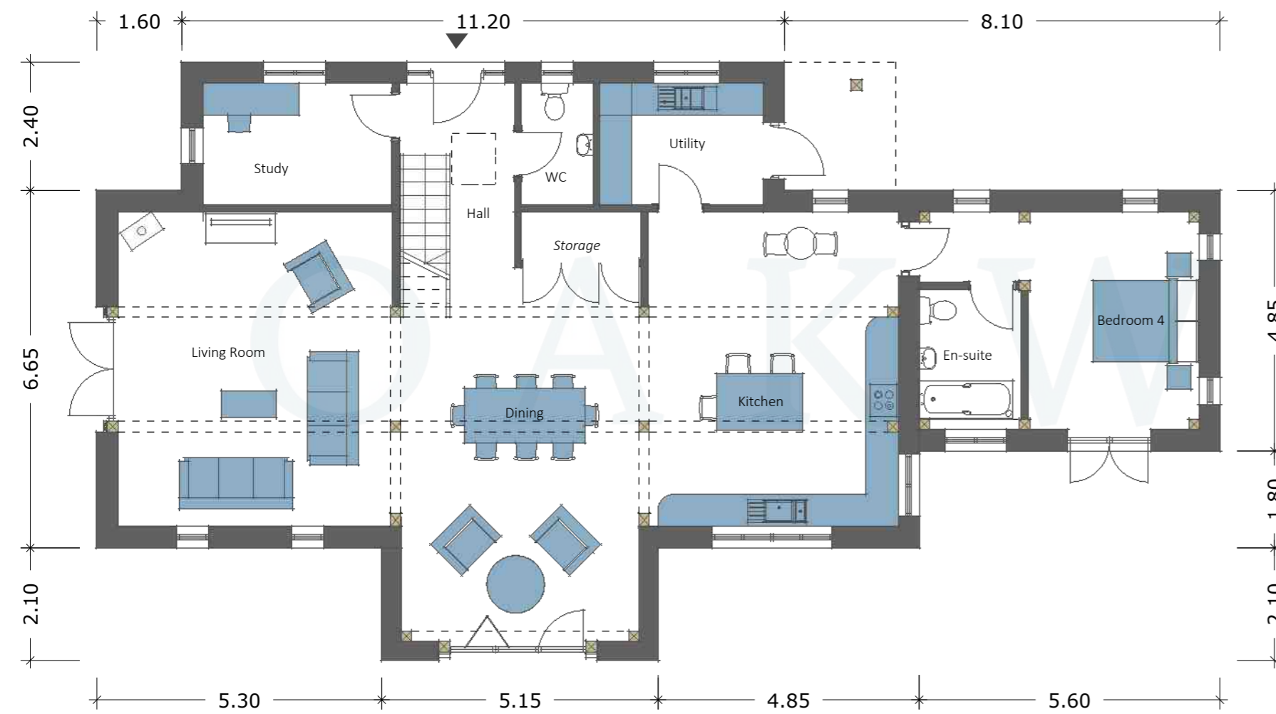
GROUND FLOOR GEA- 170.50 m 2
